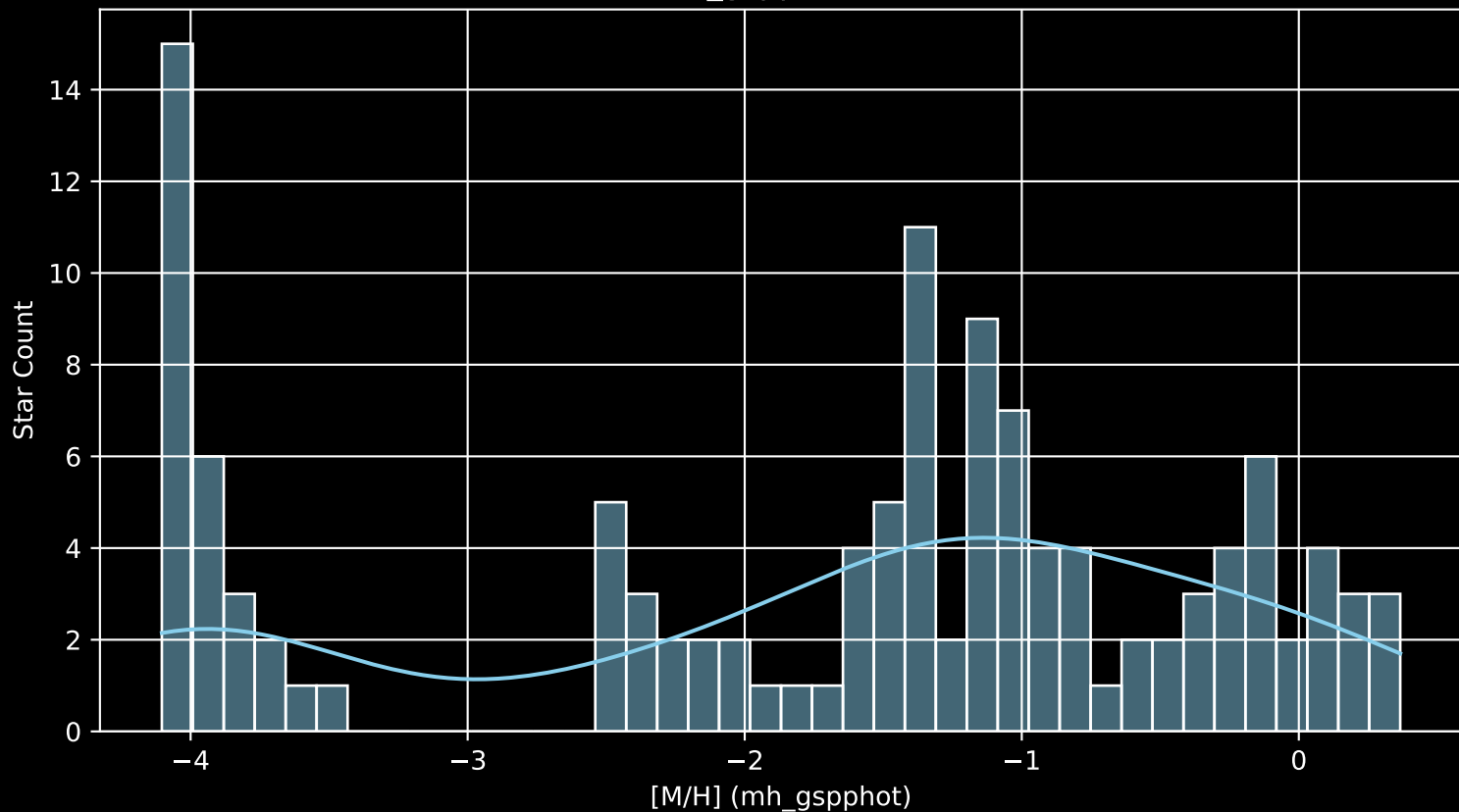
APOGEE DR17 Field: [000-03-O [M/H] (mh_gspphot) (n= 121)
