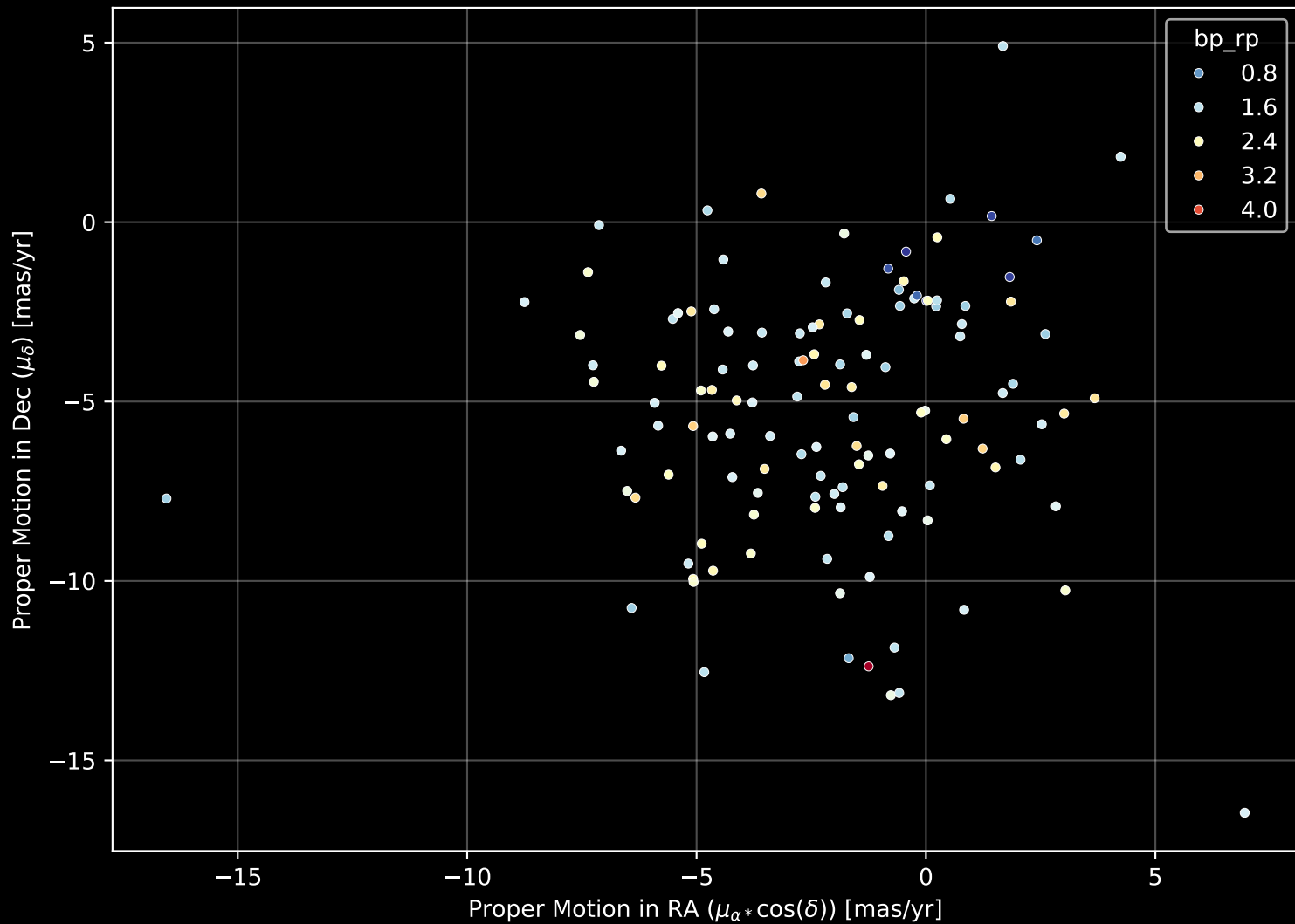
APOGEE DR17 Field: [000-03-O] Proper Motion Diagram (n= 126)
