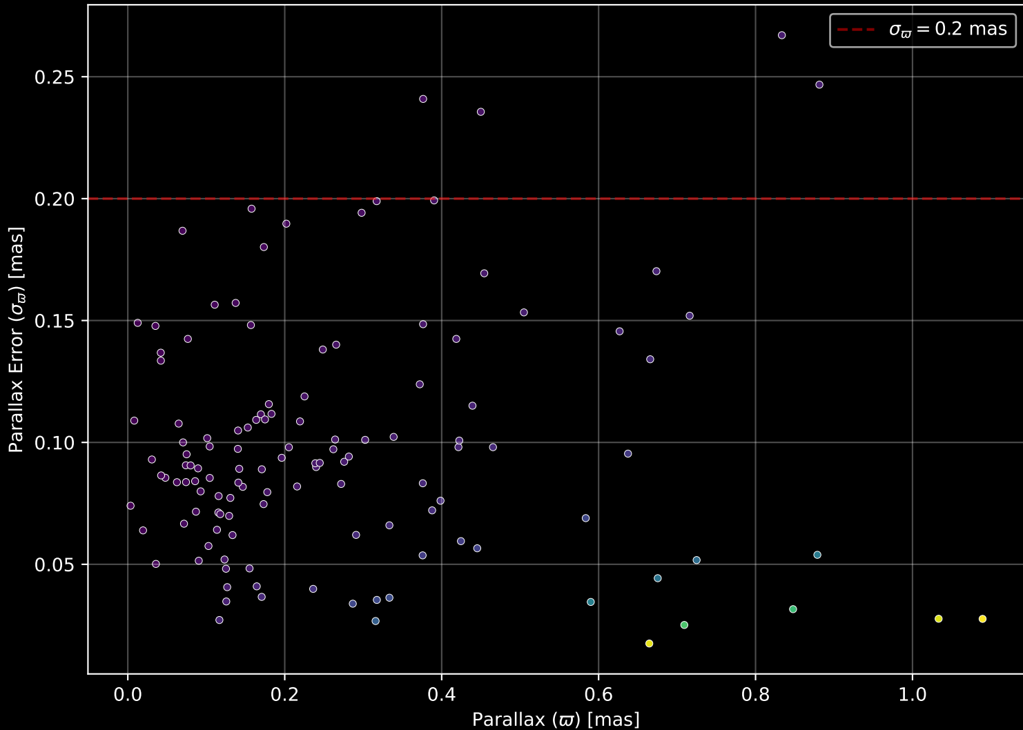
APOGEE DR17 Field: [000-03-O] Parallax Quality (n= 126)
