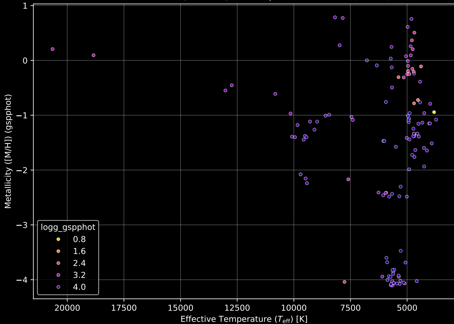
APOGEE DR17 Field: [000-03-O] Stellar Population Parameters (n= 126)
