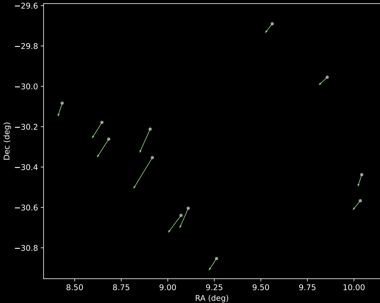
APOGEE DR17 Cluster 5 Proper Motion Vectors (n=12)
