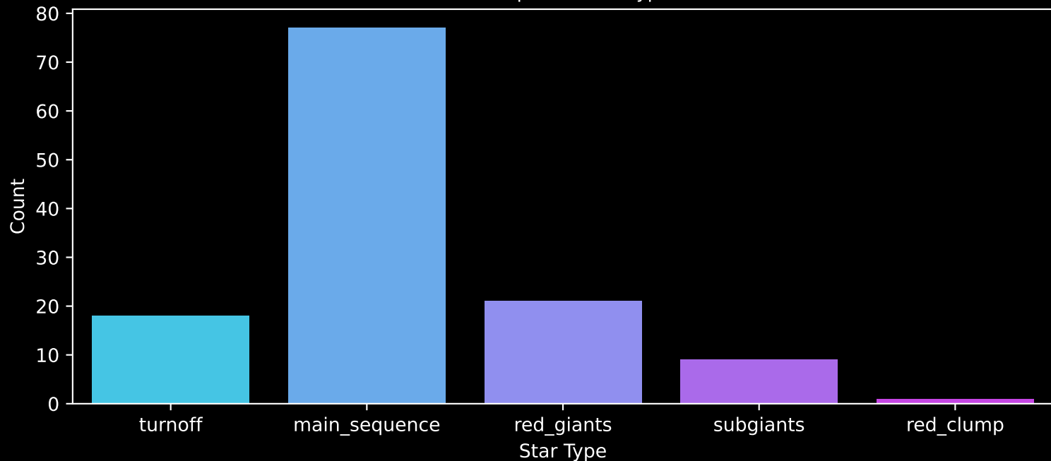
APOGEE DR17 Field: [000-03-O] Count plot of Star Type
